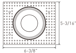
Trimless in Wood Ceiling
