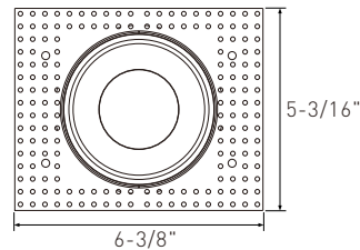
Trimless in Sheetrock and plaster only
