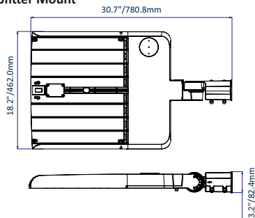
Slipfitter Mount
